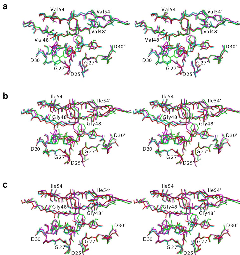
Figure 4. Binding of inhibitors in HIV-1 protease complex structures. The active site region (Asp25–Asp30), flaps (Lys45–Lys55), and the inhibitors of (a) Flap+, (b) WT, and (c) Act are superimposed and illustrated as stereo pairs. The complexes involving APV, ATV, DRV, and SQV are distinguished in red, green, cyan, and magenta, respectively.
