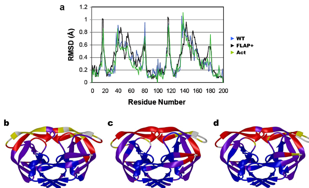
Figure 3. Structural deviation between different inhibitor complexes. (a) Distribution of root mean squared deviations (rmsd) in \alpha coordinates between the four inhibitor complexes of Flap+ (black), WT (blue), and Act (green) variants. The rmsd in \alpha coordinates in (b) Flap+, (c) WT, and (d) Act mapped on an HIV-1 protease dimer model. The color code for distinguishing the rmsd values are blue, 0–0.25 Å; purple, 0.25–0.5 Å; red, 0.5–0.65 Å; yellow, 0.65–0.8 Å; white, 0.8 Å and above.
