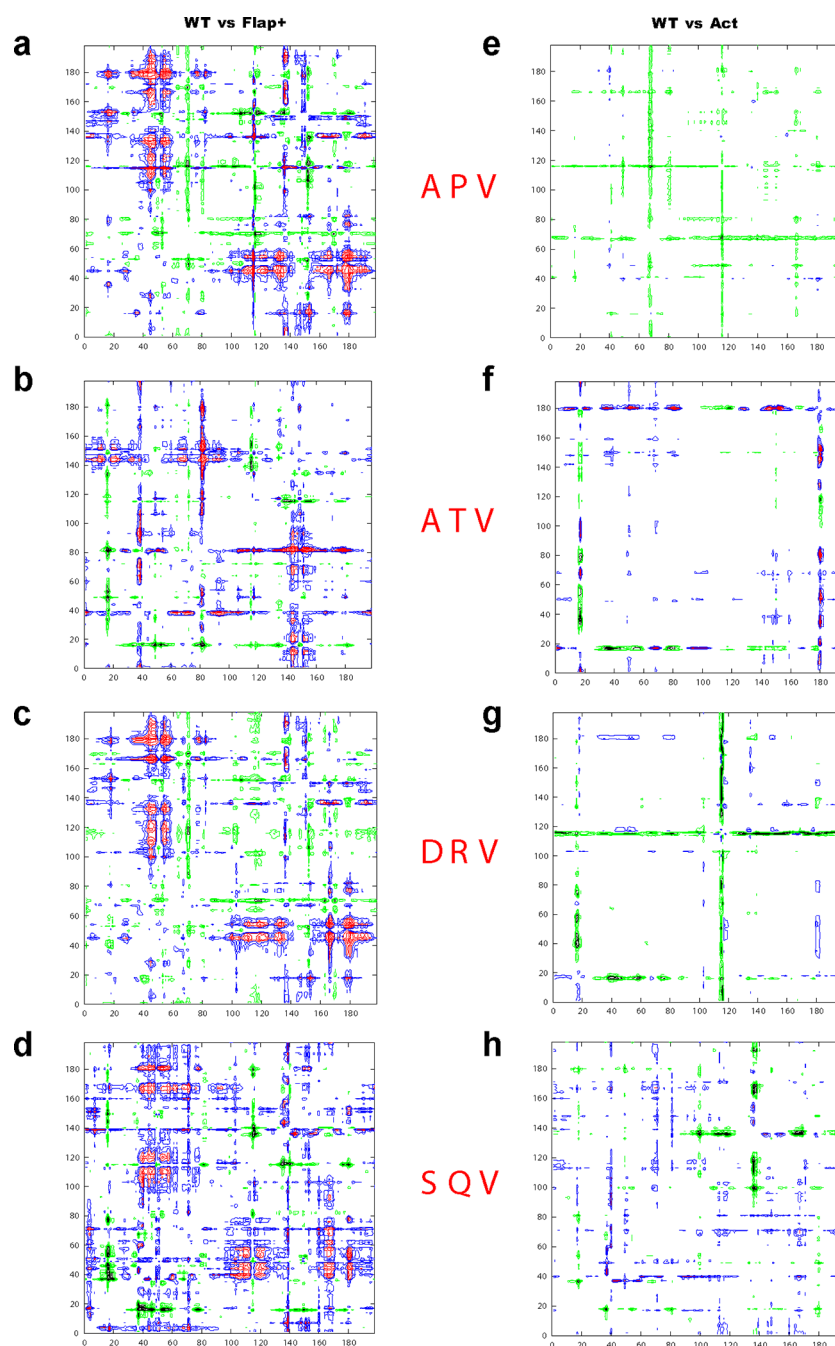
Figure 5. Comparison of mutant complex structures with WT HIV-1 protease. Double difference plots (see Methods) illustrating the WT vs Flap+ structural changes in (a) APV, (b) ATV, (c) DRV, and (d) SQV, and WT vs Act structural changes in (e) APV, (f) ATV, (g) DRV, and (h) SQV. The key for contours: (i) black -5.0 to -1.0 Å and green -1.0 to -0.5 Å (corresponding residue distances in the mutant structures have increased); (ii) blue 0.5 to 1.0 Å and magenta 1.0 to 5.0 Å (corresponding distances in the mutant structures have decreased).
