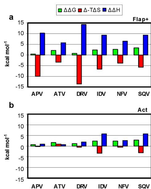
Figure 2. Thermodynamics of inhibitor binding. Differences in binding energetics between (a) WT and Flap+ and (b) WT and Act variants. The differences in \Delta G , T\Delta S , and \Delta H are shown in green, red, and blue, respectively.
